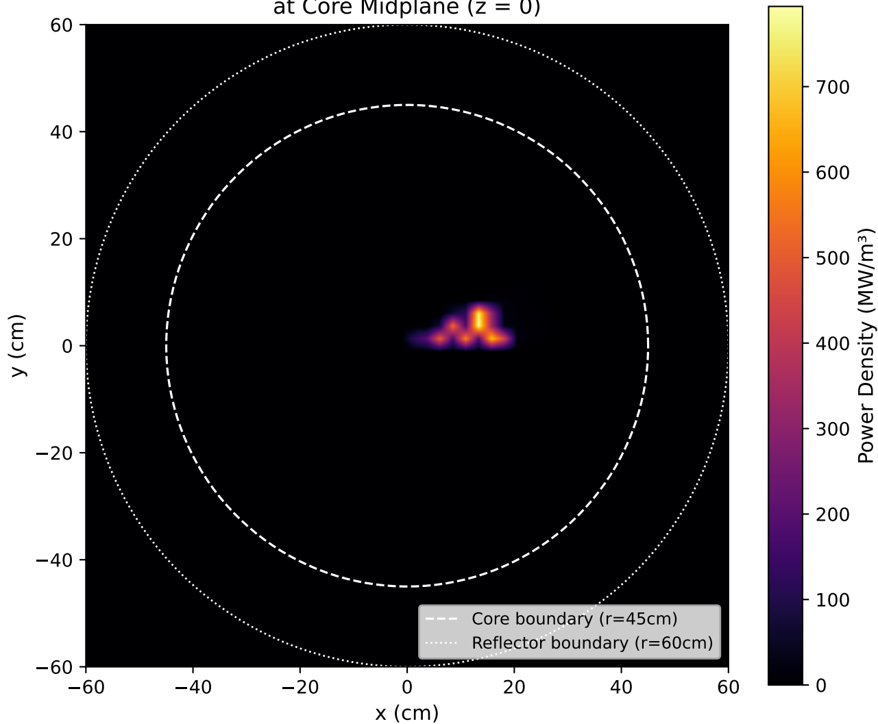
AYURI Core — Radial Power Distribution at Core Midplane ( z = 0 )
